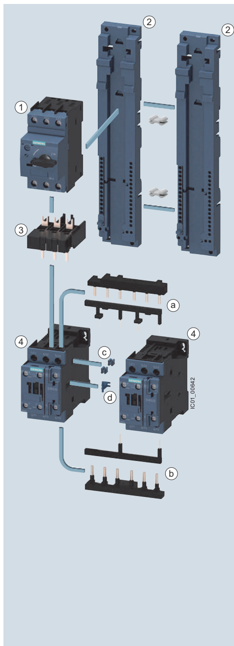
3RA22 load feeder for reversing duty and standard rail mounting in size S0 (the version with screw terminals is shown in the picture) RH assembly kits for reversing duty and standard rail mounting in size S0, see page 8/51.
