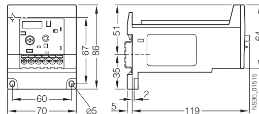
3RB30 36, 3RB31 33, size S2 with straight-through transformer
